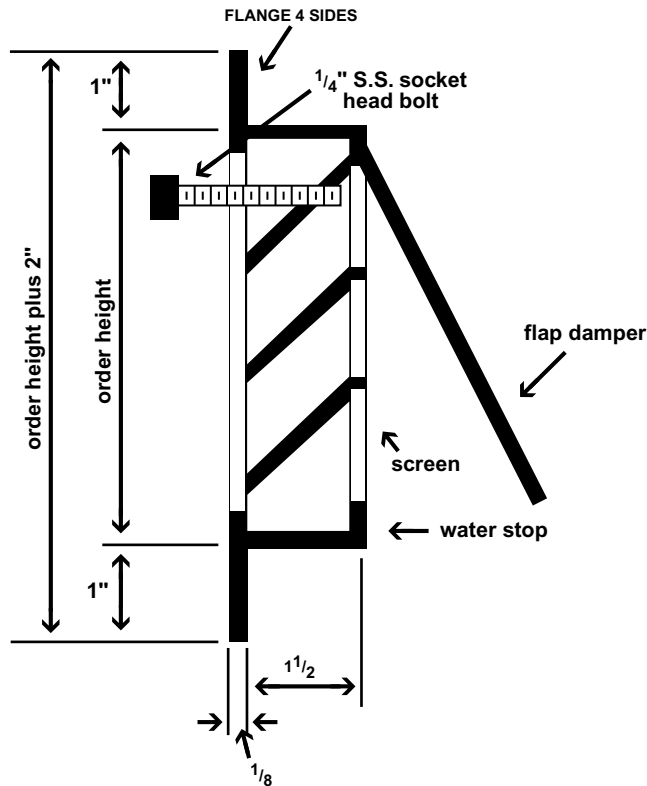
1 1/2" Deep with 1" Face Flange "FL" Vent
